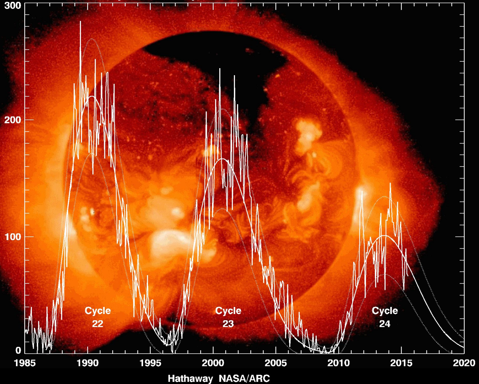
Cycle 24 Sunspot Number Prediction (2015/08)
