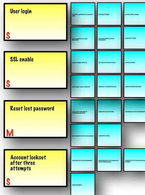
Sprint Backlog
