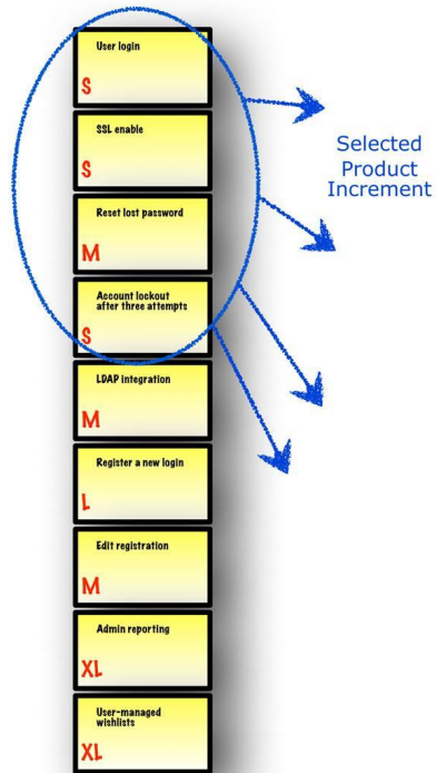
Product Backlog
