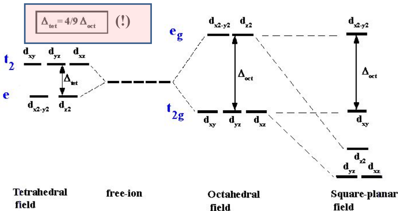
Energy levels of the d -orbitals in common stereochemistries
