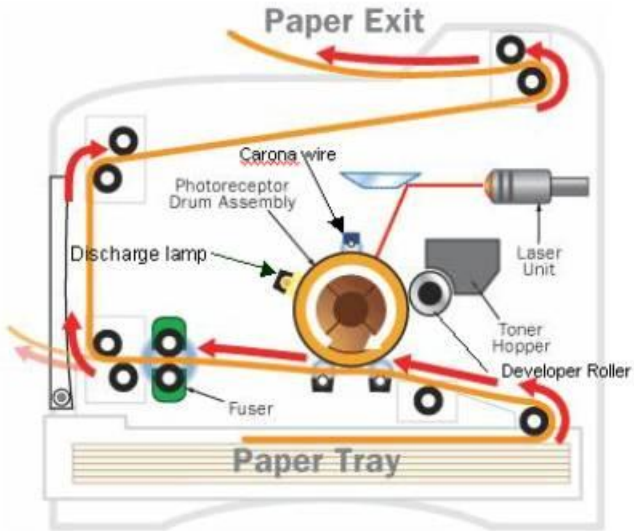
Laser printer components and their functionality
