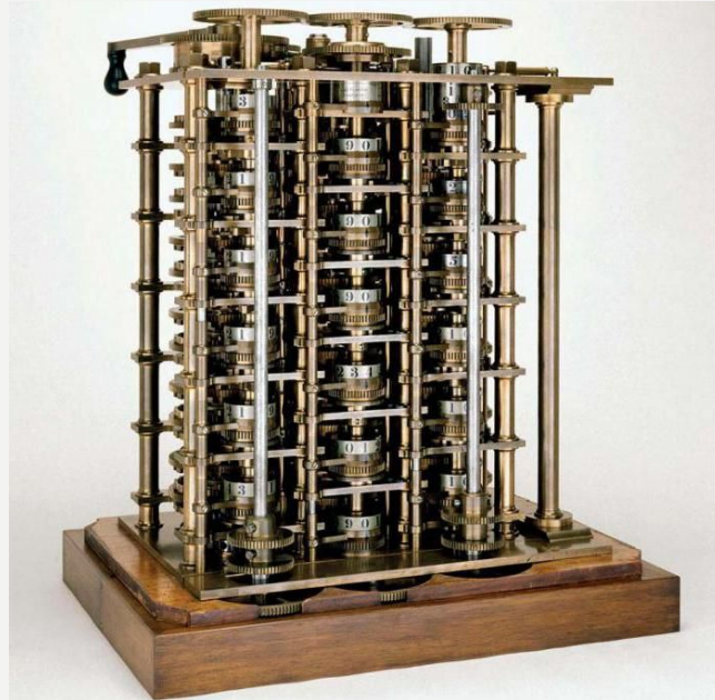
Difference Engine, 1822
