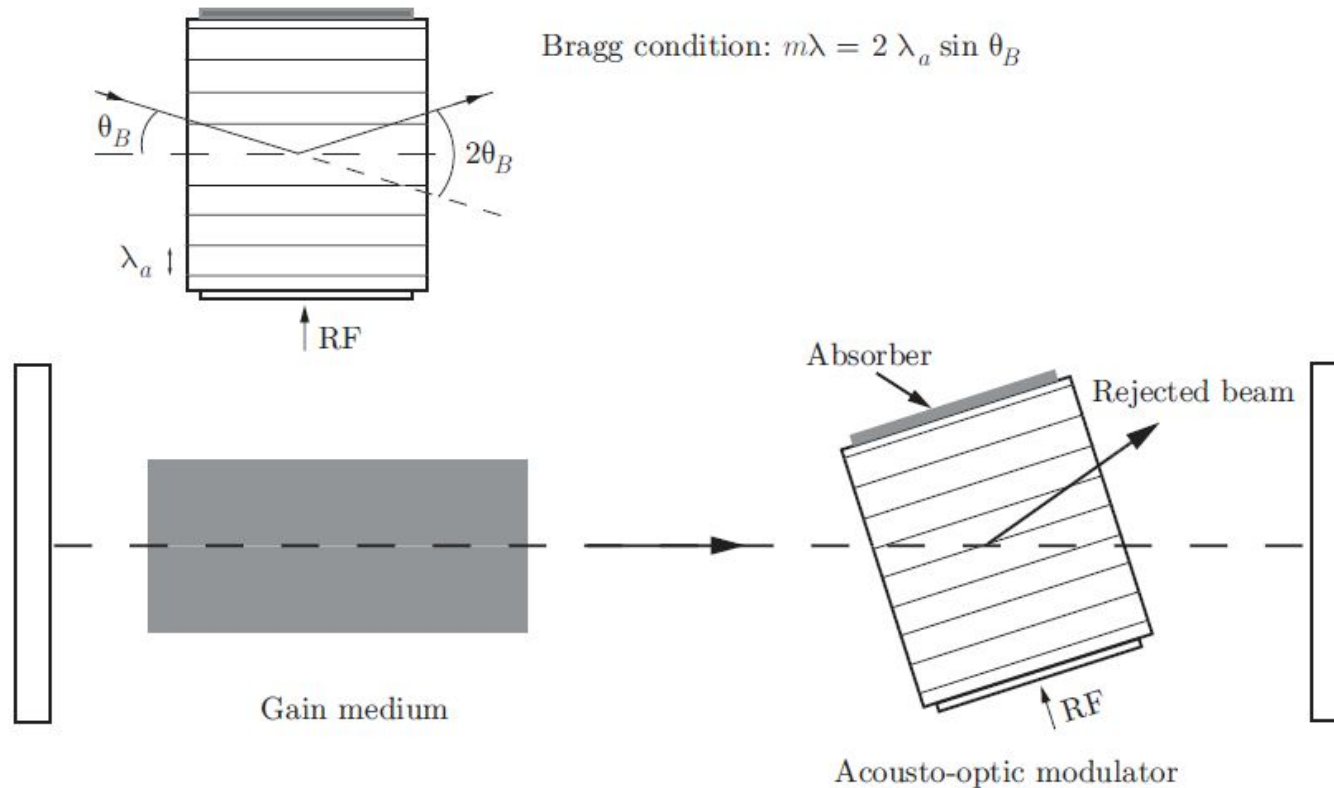
Figure 3.5: Acousto-optic Q-switching. Note that the Bragg angle \theta_B has been greatly exaggerated. A value closer to 1^\circ would be more typical. The insertion loss of the acousto-optic crystal can be eliminated (for one polarization) by rotating the crystal out of the plane of the paper through Brewster's angle.
