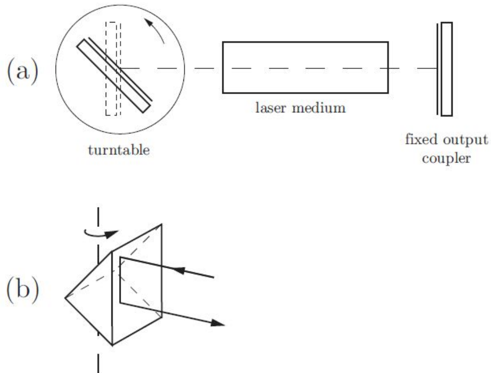
Figure 3.3: Q-switching with a rotating mirror: (a) schematic diagram of the layout of the optical cavity; (b) use of a roof prism as the rotating element. A roof prism has the advantage of automatically ensuring alignment of the reflected beam in one plane (in this case the vertical plane).
