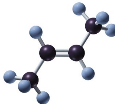
trans-
