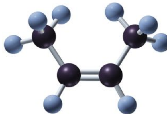
cis-
