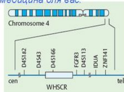
3. Scheme of physical map of 4p16
