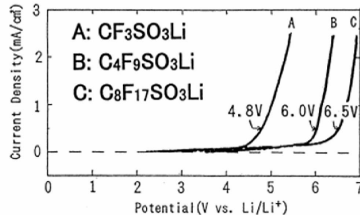
Figure 4. Potential Window of Electrolytes
