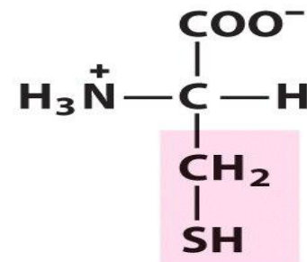
Цистеин (Cys)
