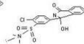
chlorthalidone
