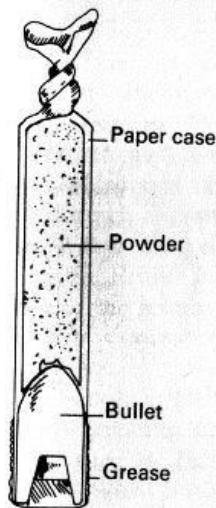
A greased cartridge
