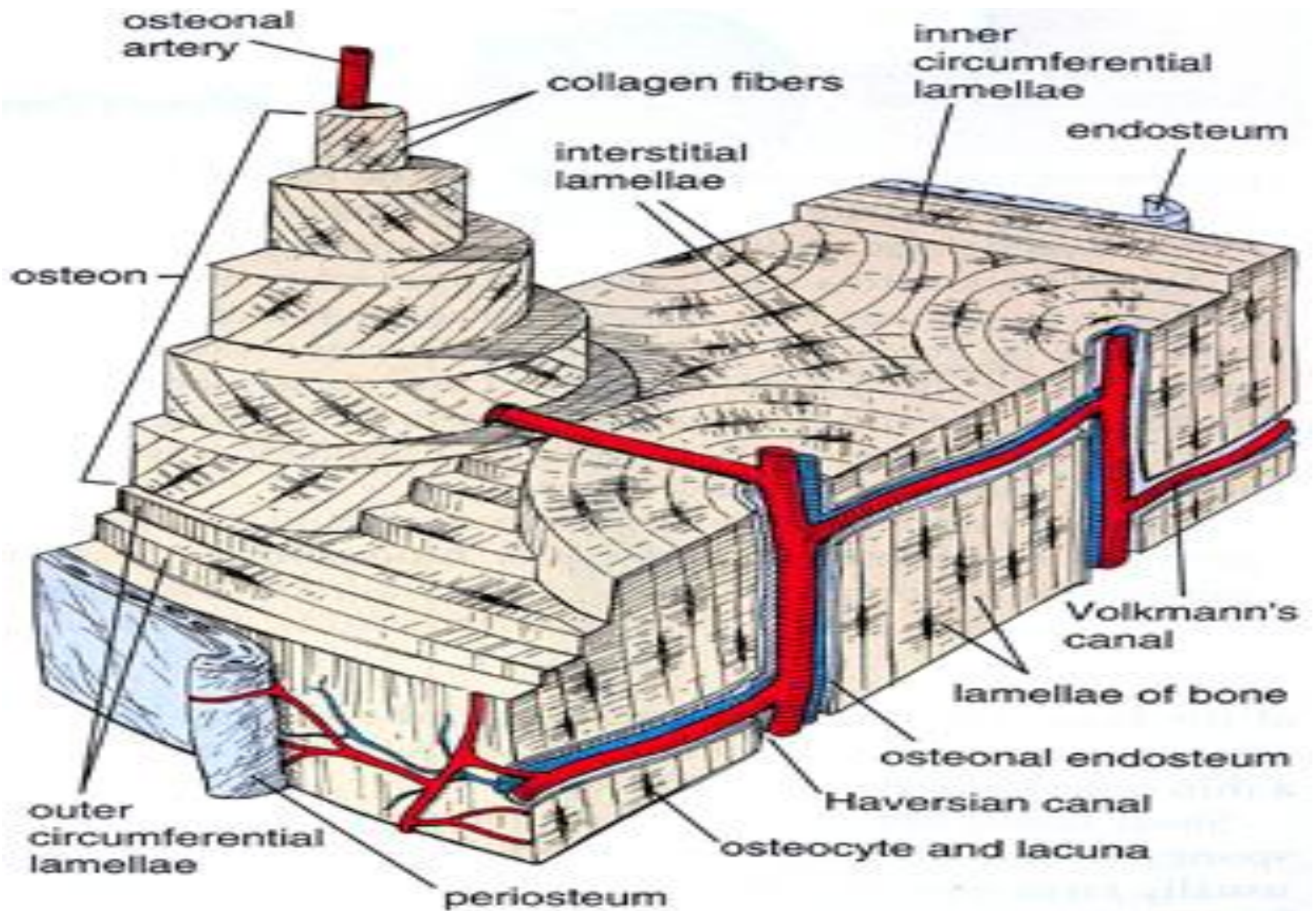
FIGURE 8.3. Diagram of a section of compact bone removed from the shaft of a long bone. The concentric lamellae and the Haversian
