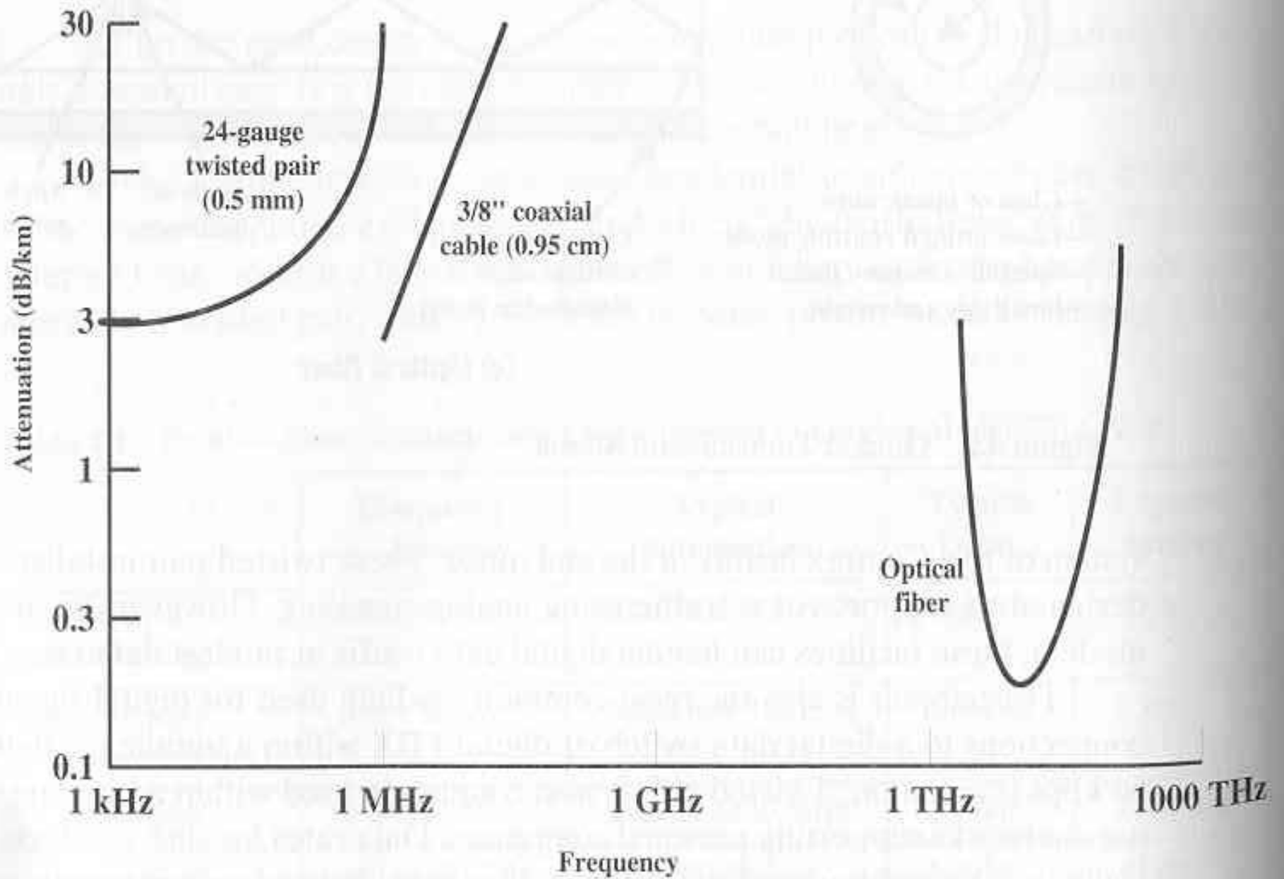
Figure 4.3 Attenuation of Typical Guided Media
