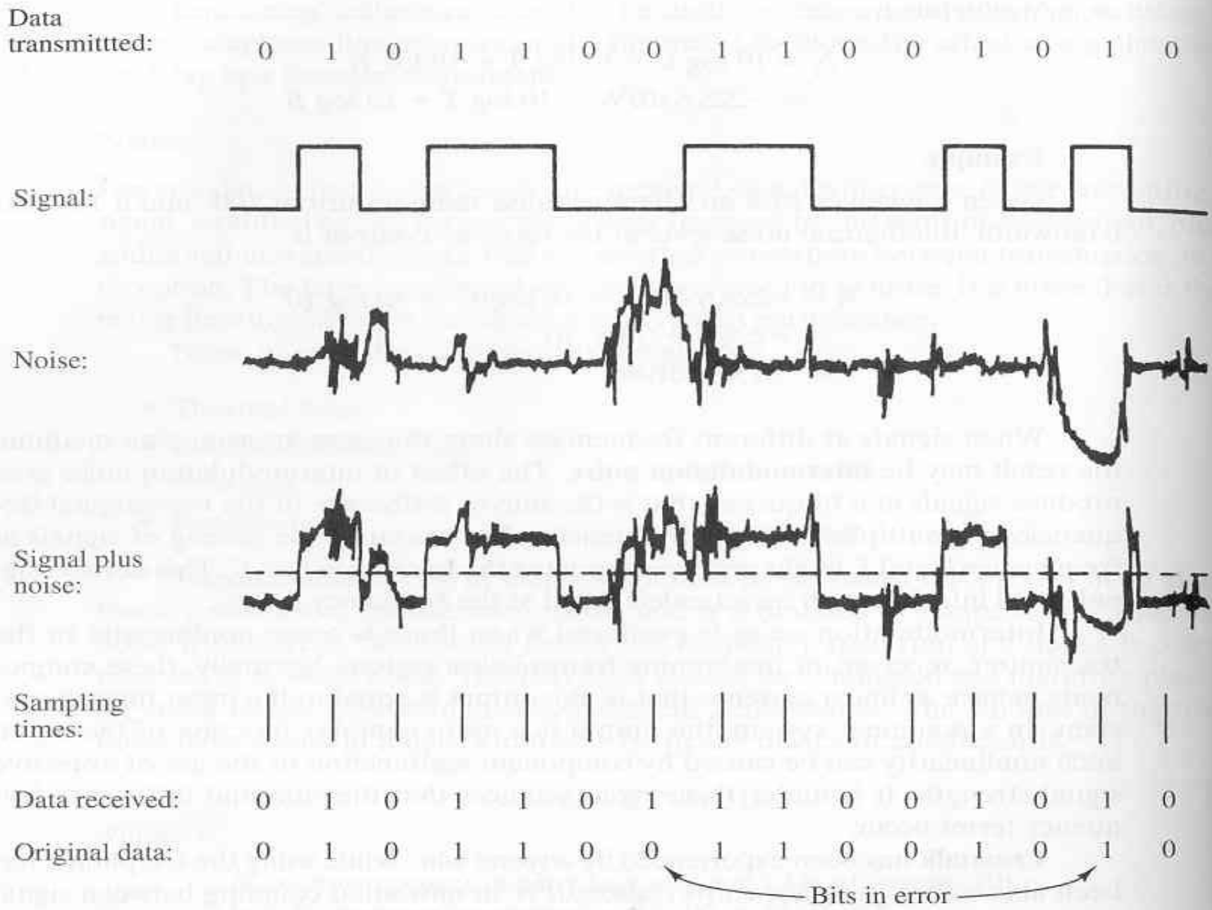
Figure 3.13 Effect of Noise on a Digital Signal.
