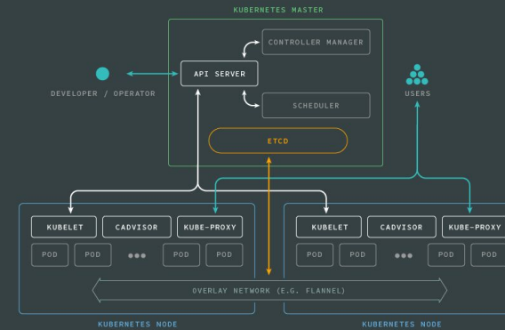
The Kubernetes Control Plane
