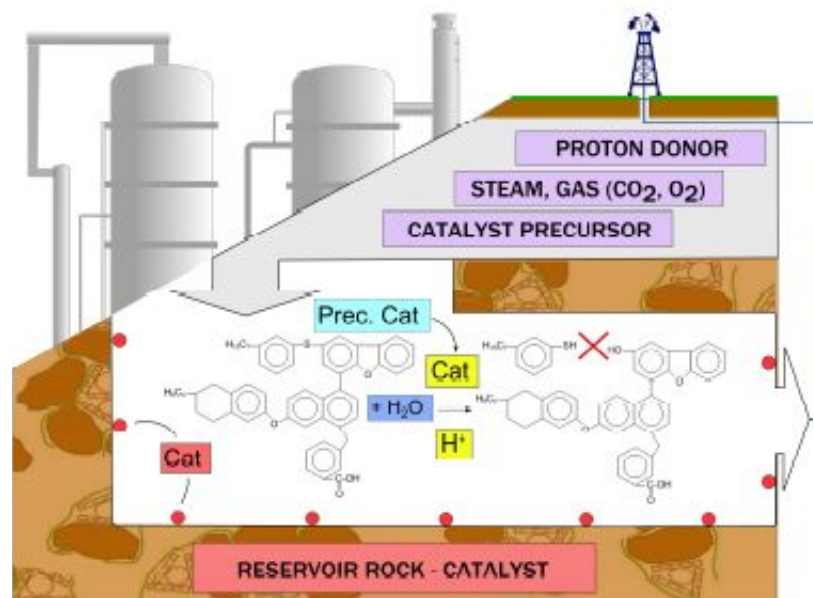
In-situ Conversion of Crude Oil Using Nano-Sized Catalysts
