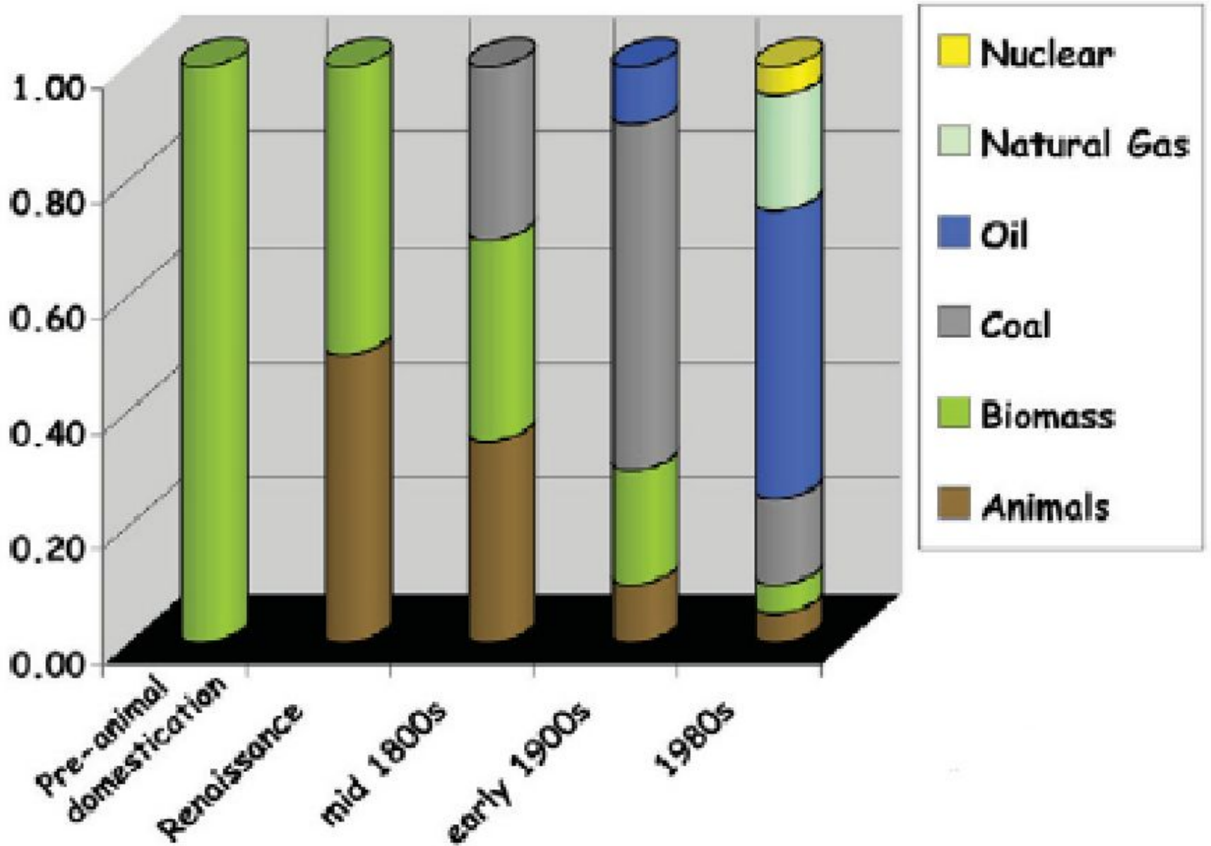
Fig. 2 Global energy sources through the ages. A simplified version of how things
