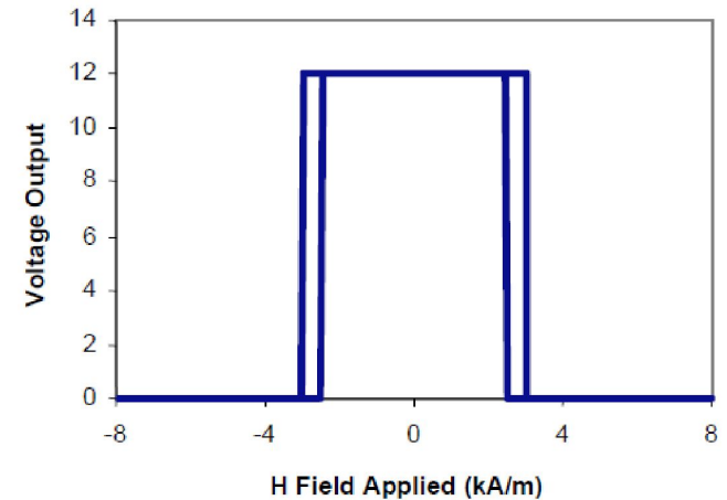
GMR Digital Switch Output
