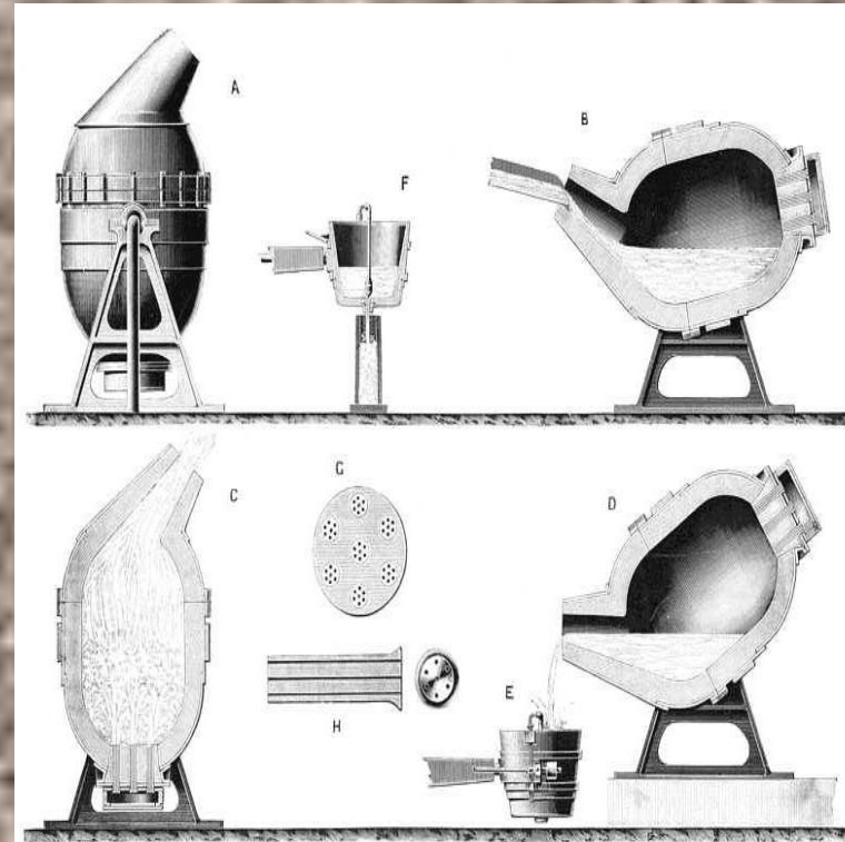
FIG. 43. THE FIRST FORM OF BESSEMER MOVEABLE CONVERTER AND LADLE
