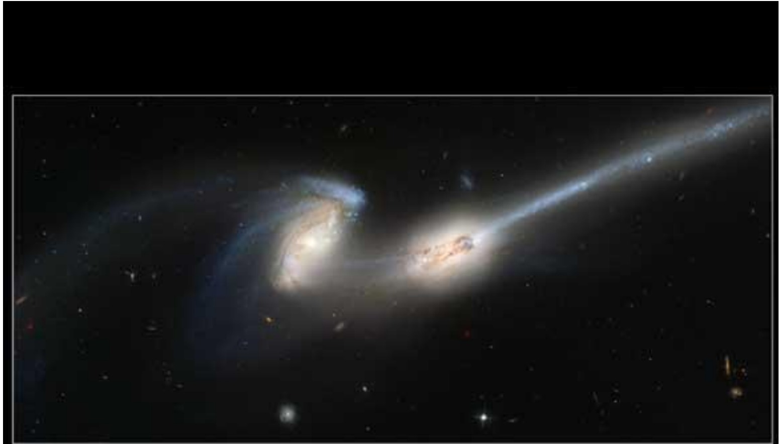
The Mice • Interacting Galaxies NGC 4676 Hubble Space Telescope • Advanced Camera for Surveys
