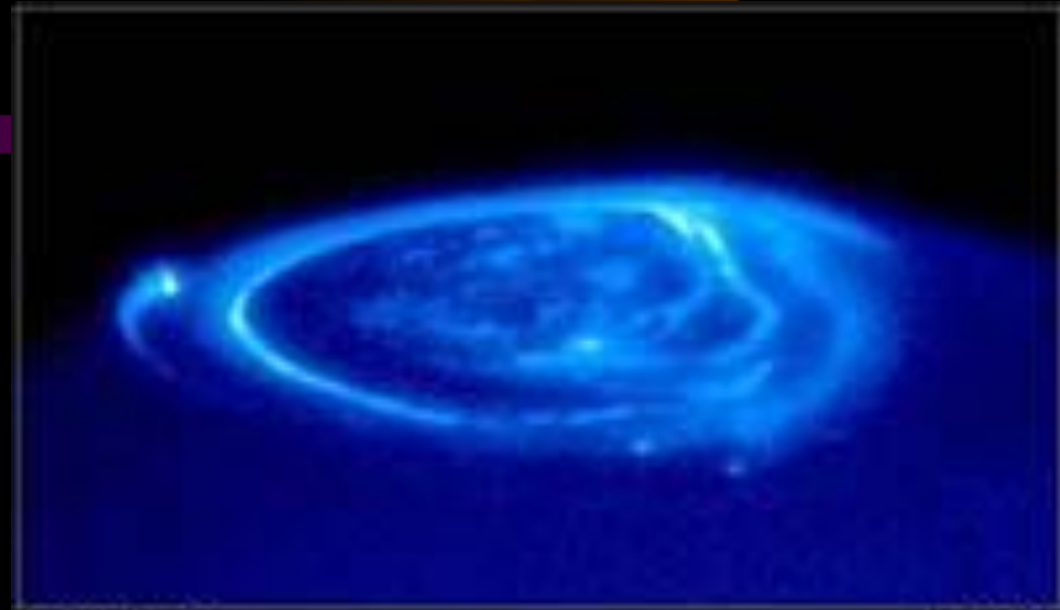
Jupiter Aurora NASA and J. Clarke University of Michigan - STScl PR02-38
