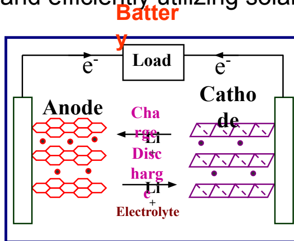
Storage Device
