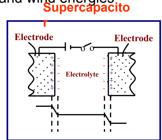
Storage Device
