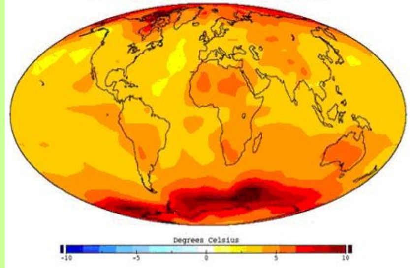
Surface Air Temperature Increase 1960 to 2060
