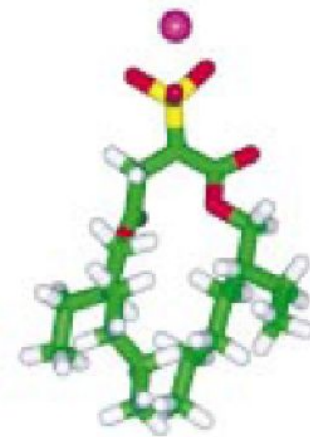
Conformer 4
