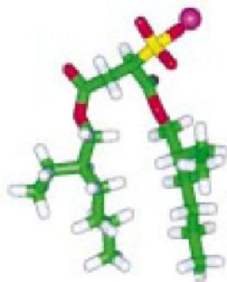
Conformer 2
