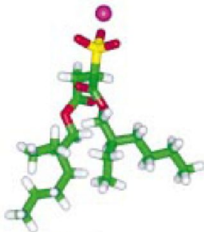
Conformer 1
