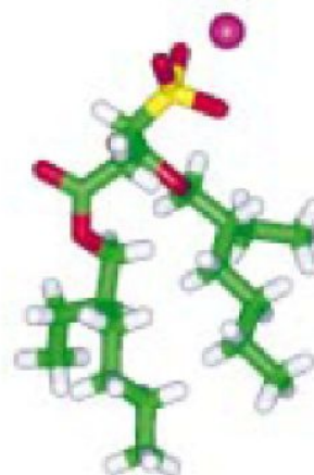
Conformer 3
