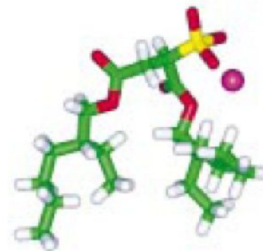
Conformer 4
