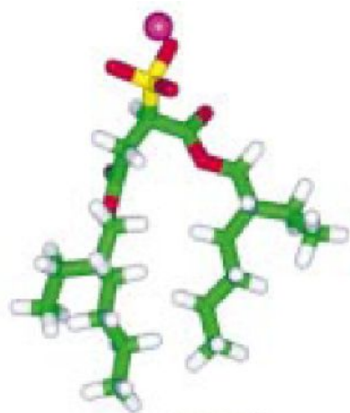
Conformer 1
