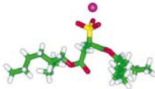
Conformer 2
