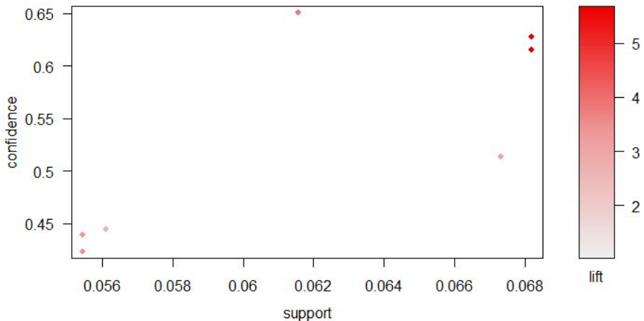
Scatter plot for 7 rules
