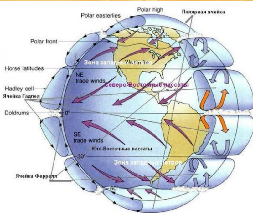
Figure 8•3 Idealized global circulation proposed for the three-cell circulation model.
