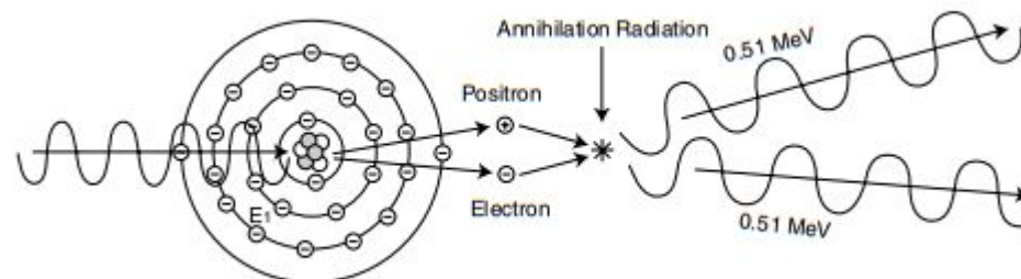
d) Pair Production
