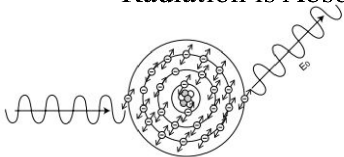
b) Rayleigh or Coherent Scattering
