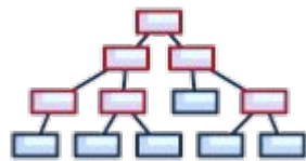
Composite
