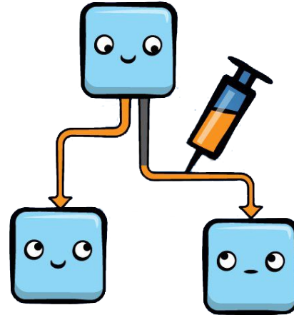
Dependency Injection
