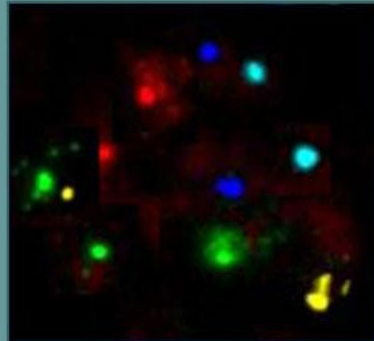
Trisomy 21
