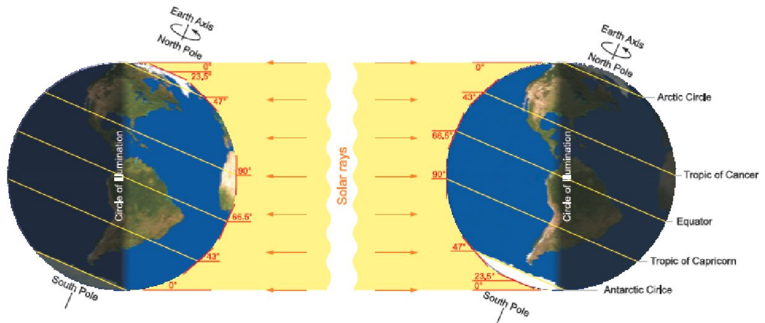
2.16 SOLSTICE CONDITIONS Because of the tilt of the Earth's axis, polar regions experience either 24-hour daylight or 24-hour darkness. The subsolar point lies on the Tropic of Cancer (lat. 23\frac{1}{2}^{\circ} N) in June (left) and on the Tropic of Capricorn (lat. 23\frac{1}{2}^{\circ} S) in December (right). (From Introduction to Weather and Climate by O.W. Archibold, John Wiley & Sons Canada, Ltd., 2011.)
