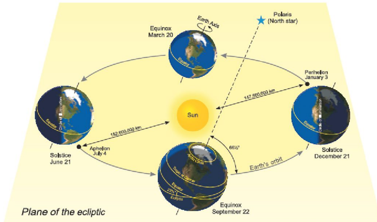
2.13 REVOLUTION OF THE EARTH Viewed from a point over the North Pole, the Earth both rotates and revolves in a counter-clockwise direction. Earth is closest to the sun at perihelion, and furthest from the sun at aphelion (relative distances are greatly exaggerated). (From Introduction to Weather and Climate by O.W. Archibold, John Wiley & Sons Canada, Ltd., 2011.)
