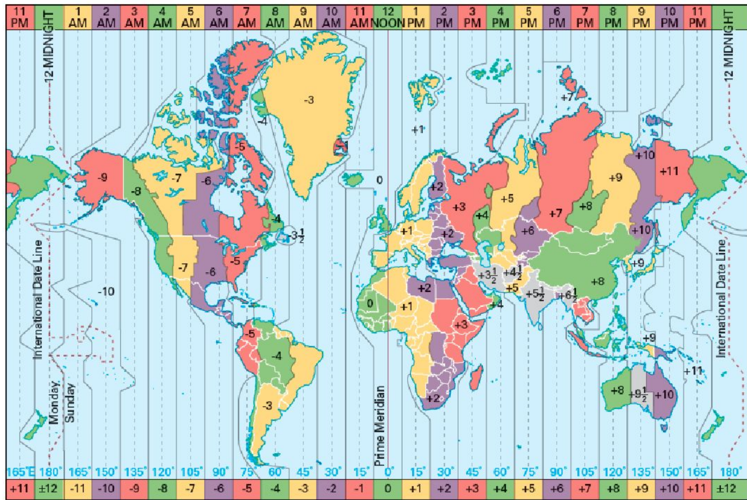
2.10 TIME ZONES OF THE WORLD Dashed lines represent 15° meridians, and bold lines represent 7½° meridians. Alternate zones appear in colour. (After U.S. Navy Oceanographic Office.)
