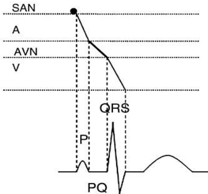
FIGURE 1-1. From the SAN, the impulse travels along preferential pathways made up of specialized fibrous cells to the atria (A), AVN, His bundle and its branches, and finally to the ventricular myocardium (V). This sequence of electrical activation occurs in little more than 200 ms; on the surface ECG, it generates the P wave, the PR interval, and the QRS complex in succession.
