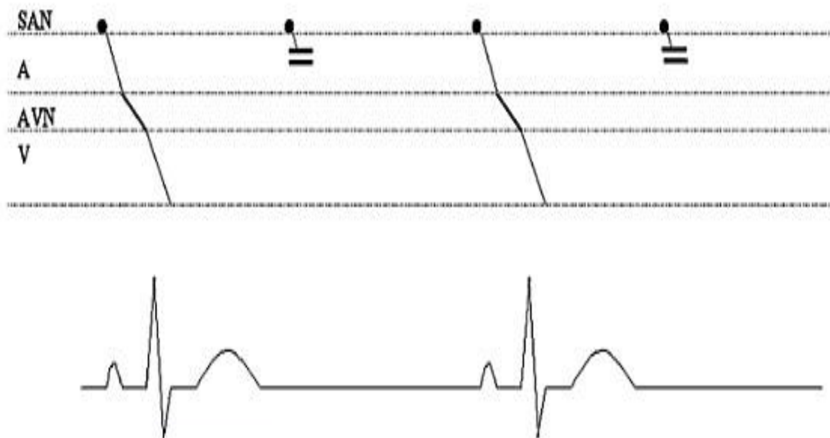
FIGURE 1-4. 2:1 sinoatrial block is characterized by the lack of conduction to the atria of each alternate impulse (on surface ECG, bradycardia is indistinguishable from sinus bradycardia due to reduced SAN automaticity).
