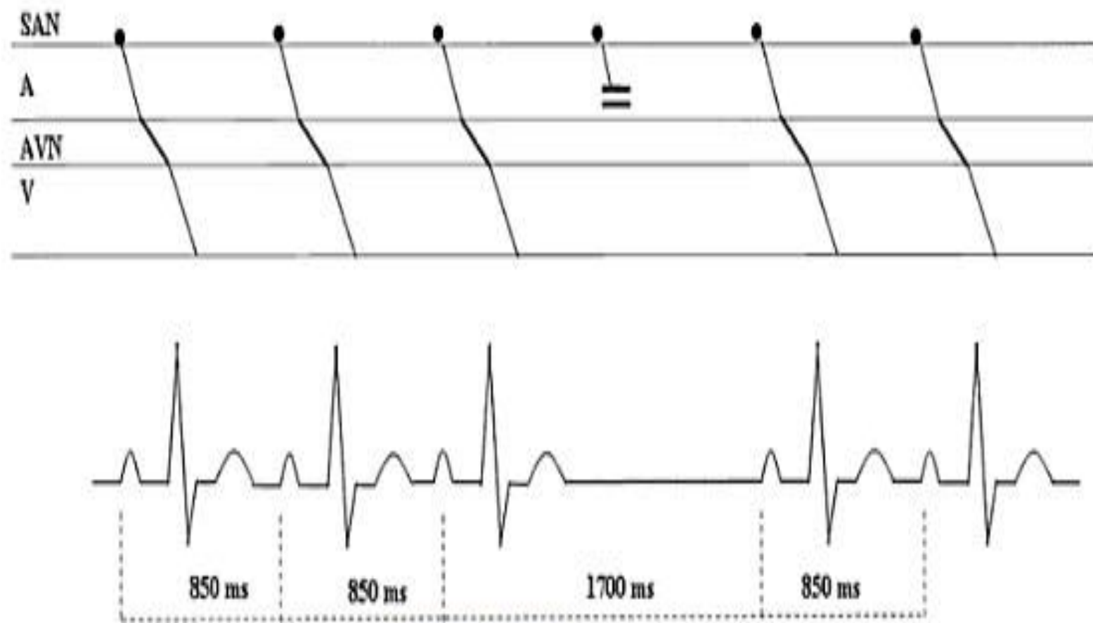
FIGURE 1-3. Second-degree Mobitz sinoatrial block . Sudden lack of conduction of a sinus impulse without progressive lengthening of conduction time.
