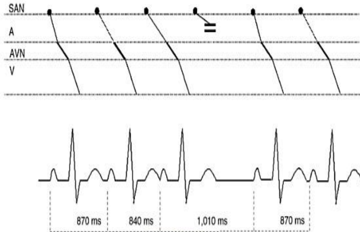
FIGURE 1-2. Second-degree Wenckebach sinoatrial block . Propagation of the impulse from the SAN to the atria progressively slows down and is finally interrupted.
