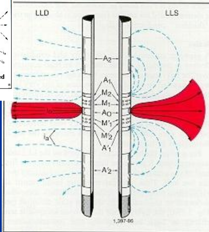
Fig. 7-13—Schematic of the Dual Laterolog.
