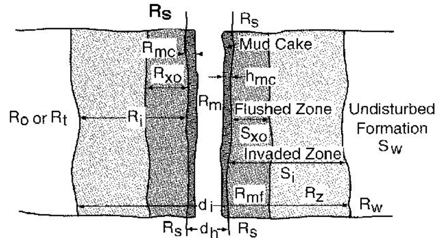
Lateral View Across Borehole
