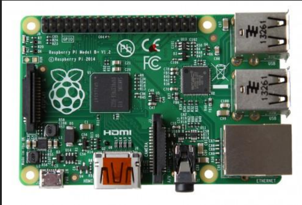
Raspberry pi 3 B+ 86.9mm x 58.5mm x 19.1mm
