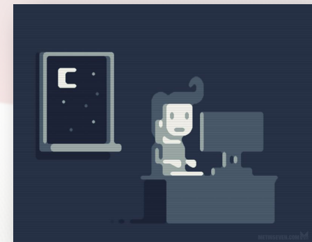
Programming
