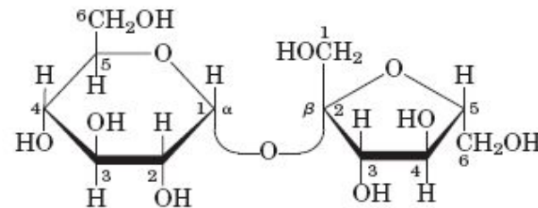
Sucrose
