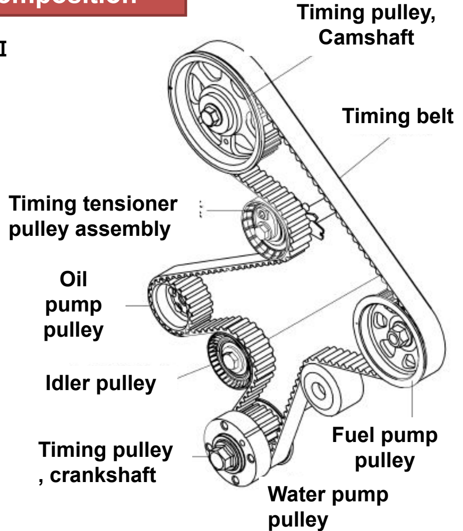
Timing system diagram
