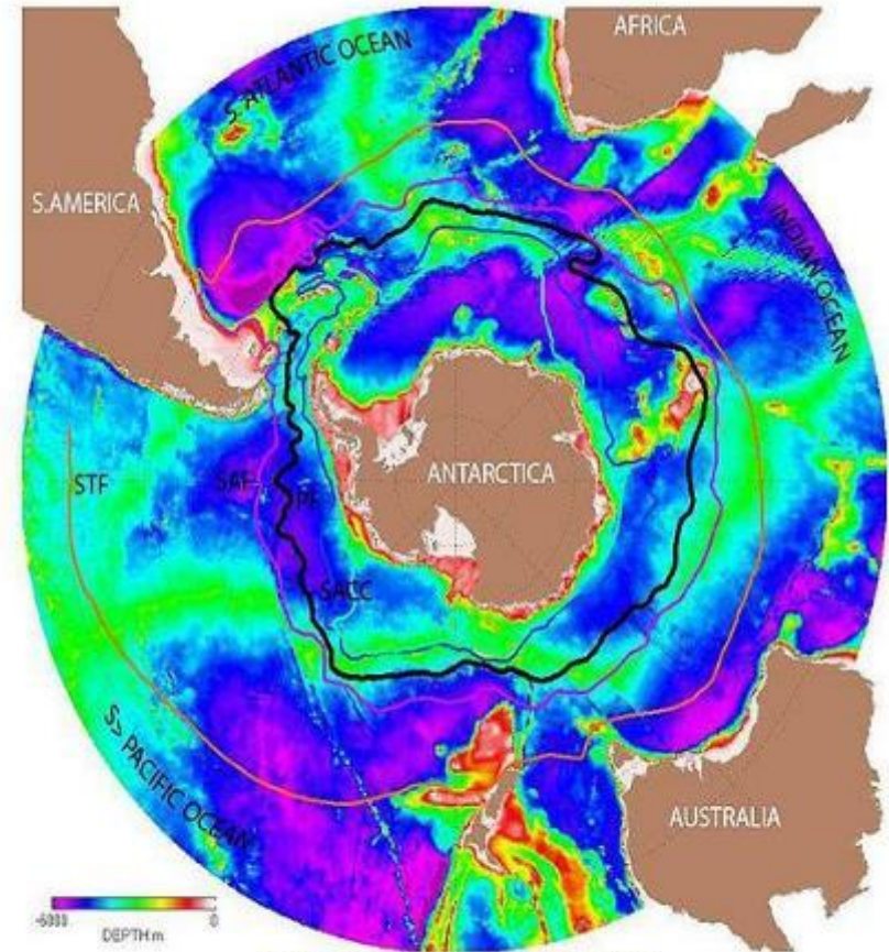
ANTARCTIC CIRCUMPOLAR CURRENT SEAWATER DENSITY FRONTS (FROM ORSI et al, 1995), AND BATHYMETRY OF THE SOUTHERN OCEAN (UP TO LATITUDE 25 S)
