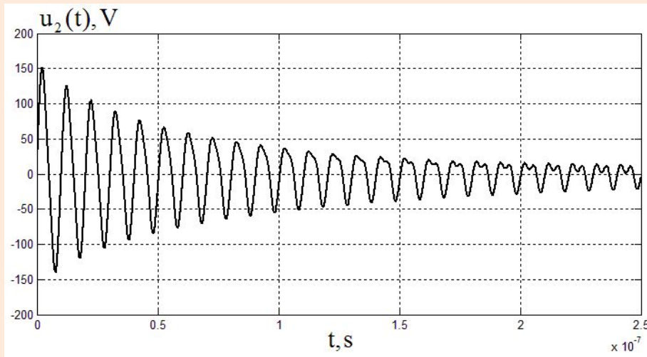
a) m_c = 0.1
