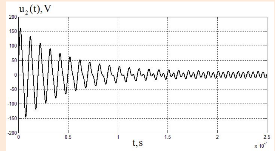
c) m_c = 0.09
