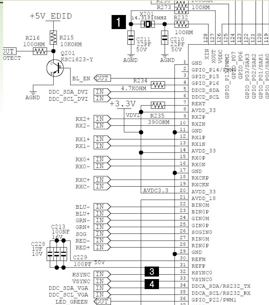
The Circuit diagram when no video (Analog)
