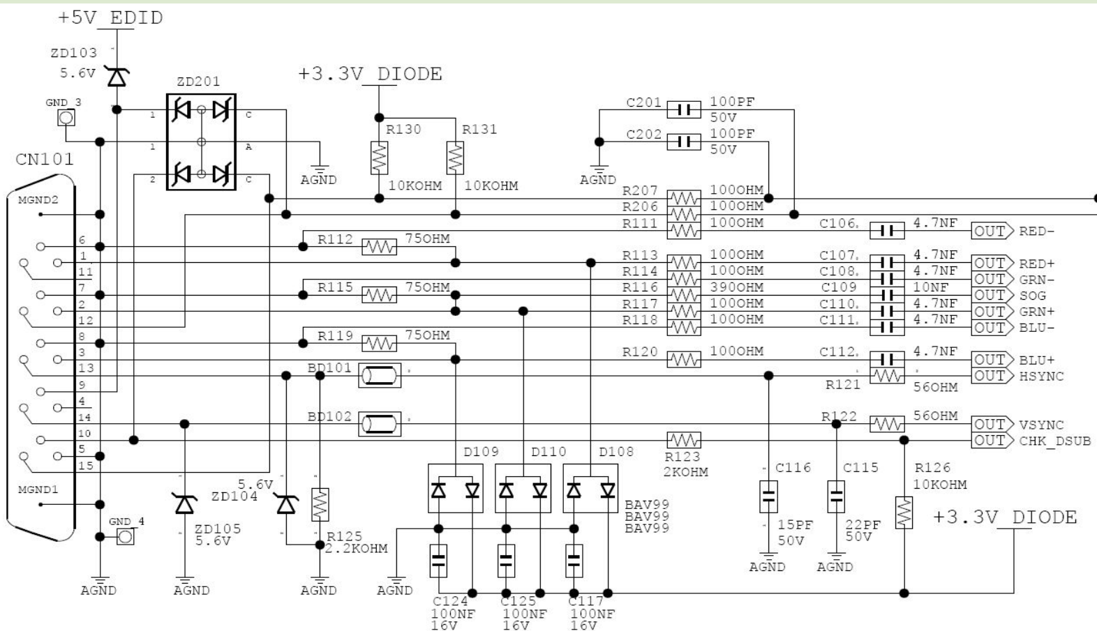
The Circuit diagram when no video (Analog)
