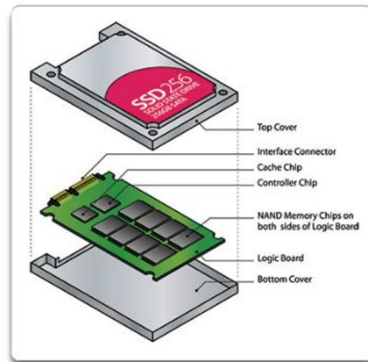
SSD Components
