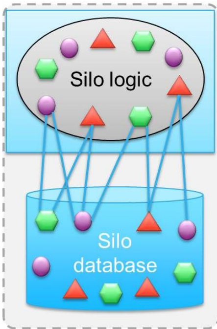
Monolithic application
