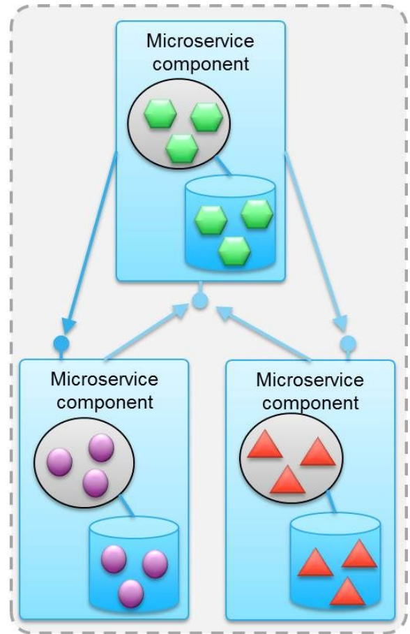
Microservices application
