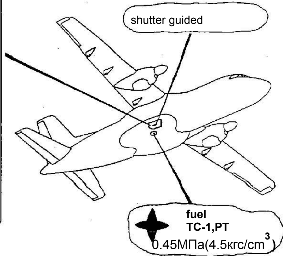
Right cowling of undercarriage
