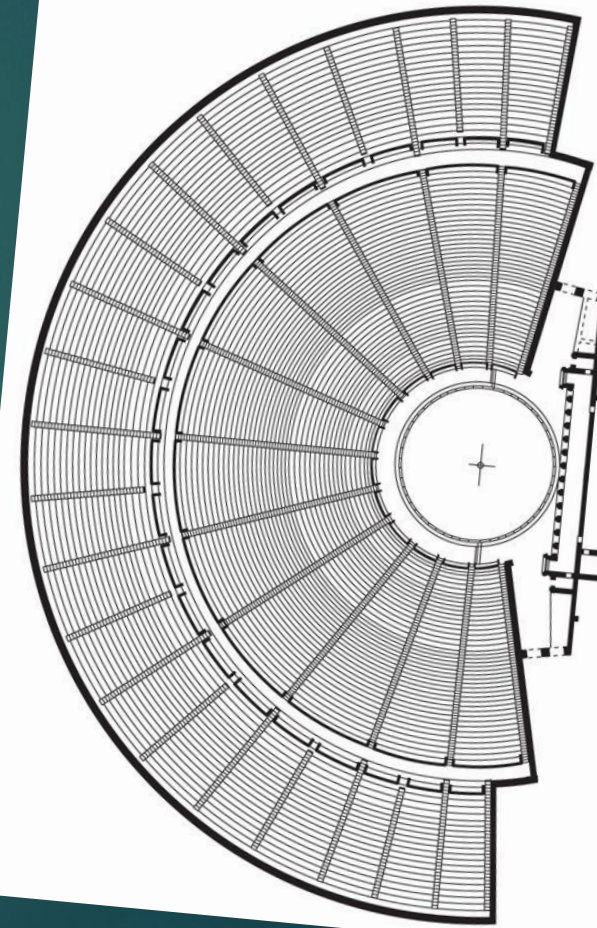
0 10 20 30 40 50 60 70 80 90 100m Epidaurus (modern Epidaurus, Greece) Cavea width: 119 m, orchestra width: 24.65 m, capacity: 11,750-14,700; ca. 300-340 BC. Plan (T.H. after Gerkan)
