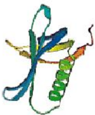
(18) 1prtF:1 OB-fold
