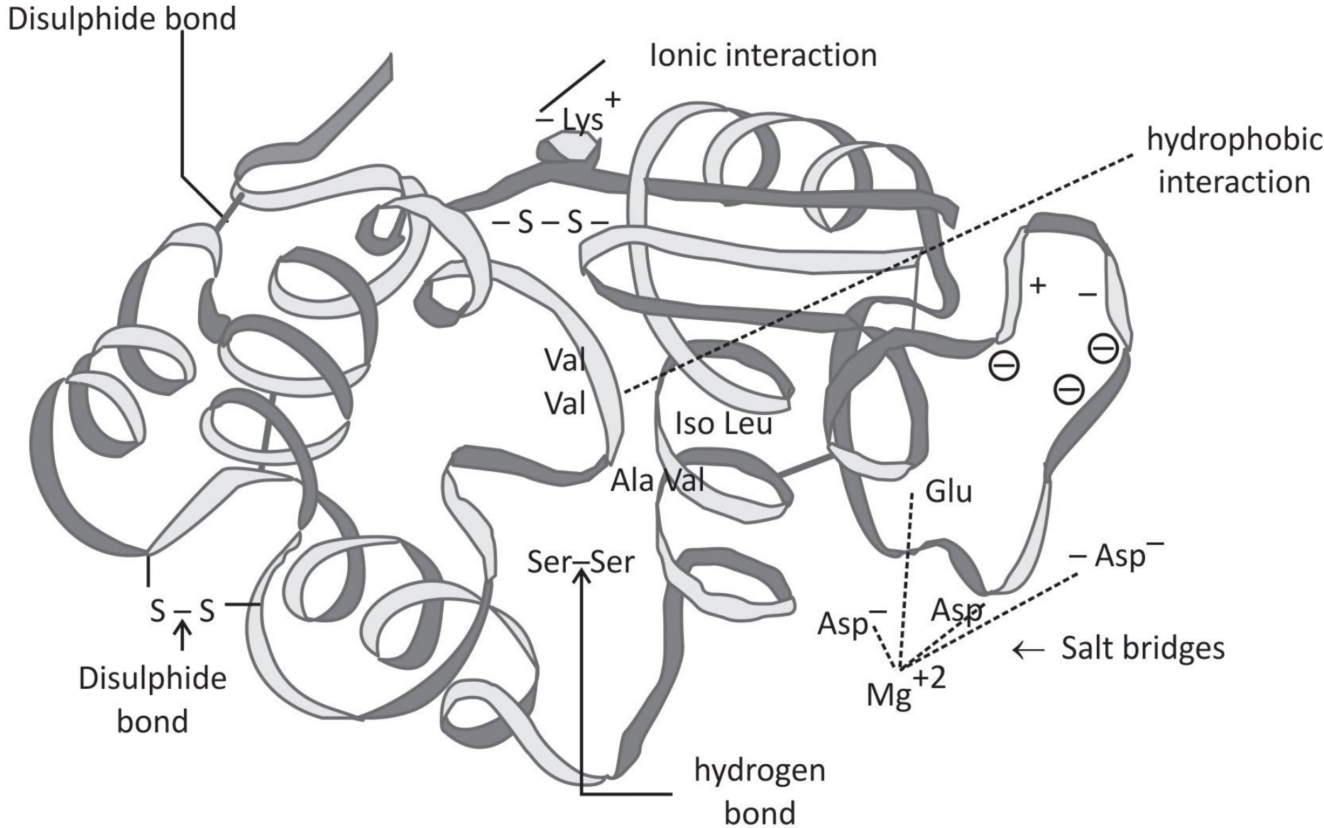
Fig. : Tertiary Structure of protein involving various forces.
