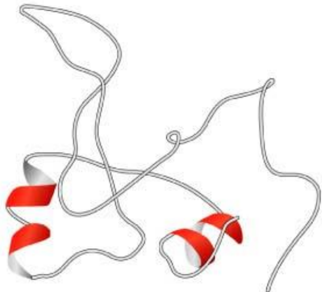
(a) denatured
