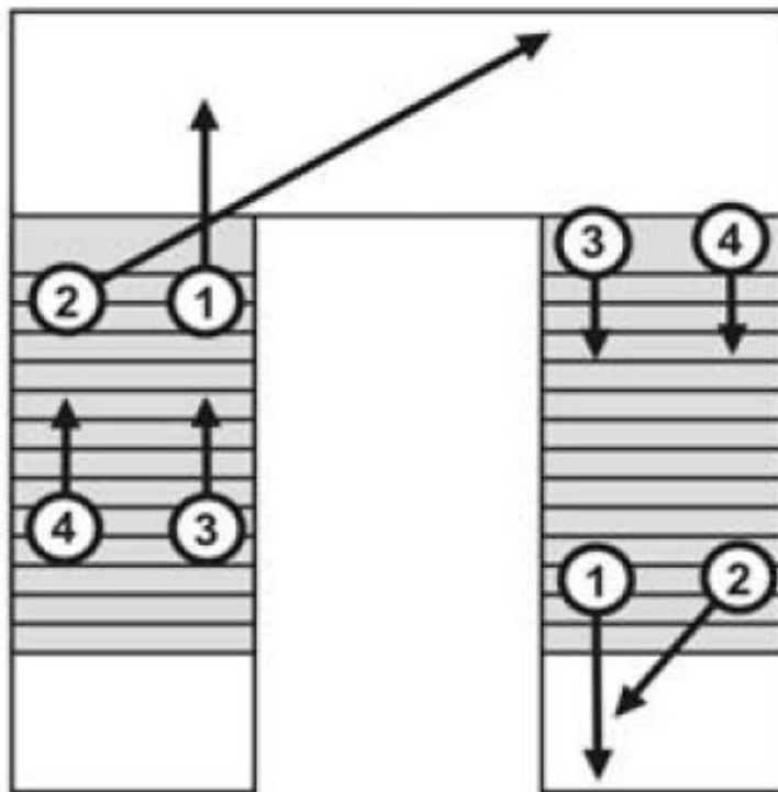
Figure 6-17. CLOSED STAIRWELL
