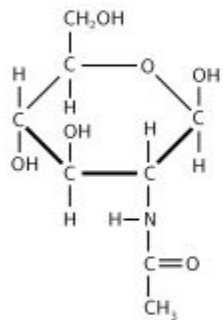
N-Acetyl-Glucosamin
