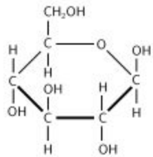
Beta-D-Glucose
