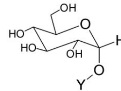
Glycolipids
