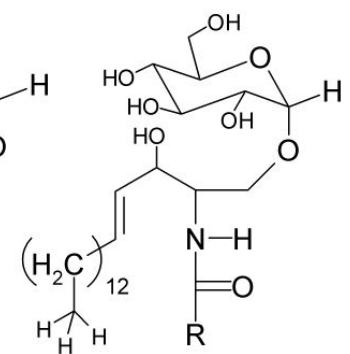
Sphingo-Glycolipids
