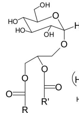
Glycero-Glycolipids
