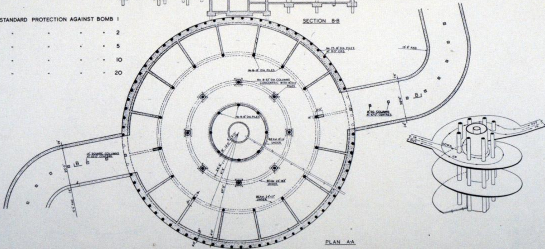
Drawing No. 16.
