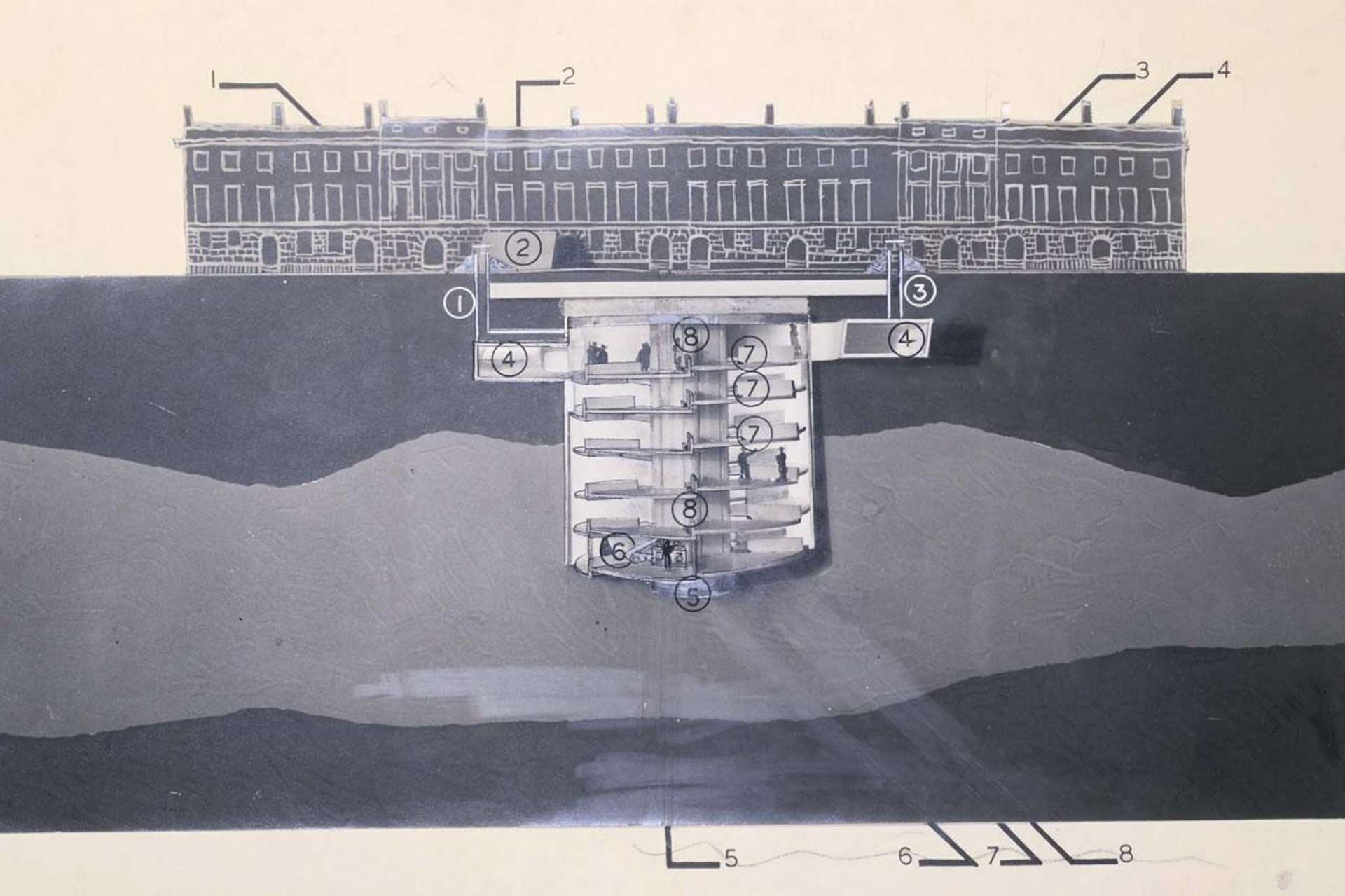
Berthold Lubetkin, Tecton group, deep shelter for 7600 people
