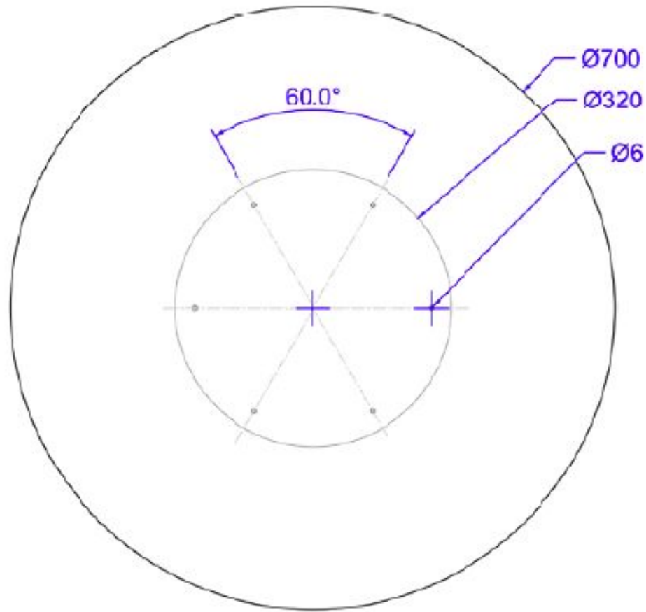
TOP VIEW
