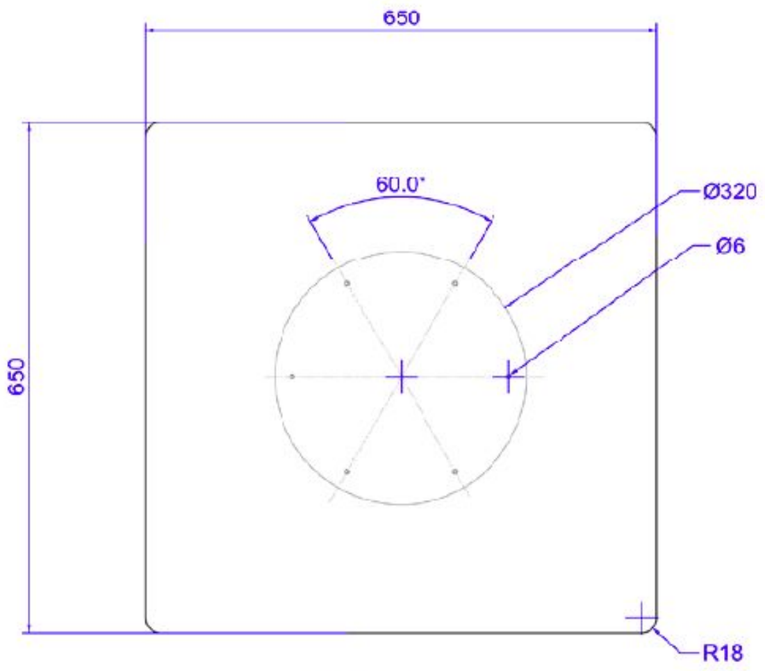
TOP VIEW
