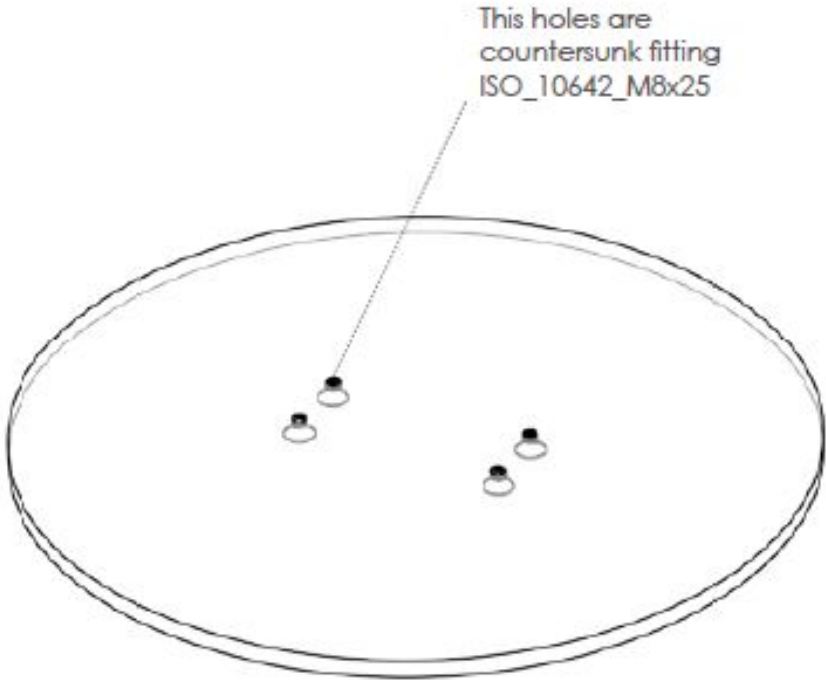
PERSPECTIVE
