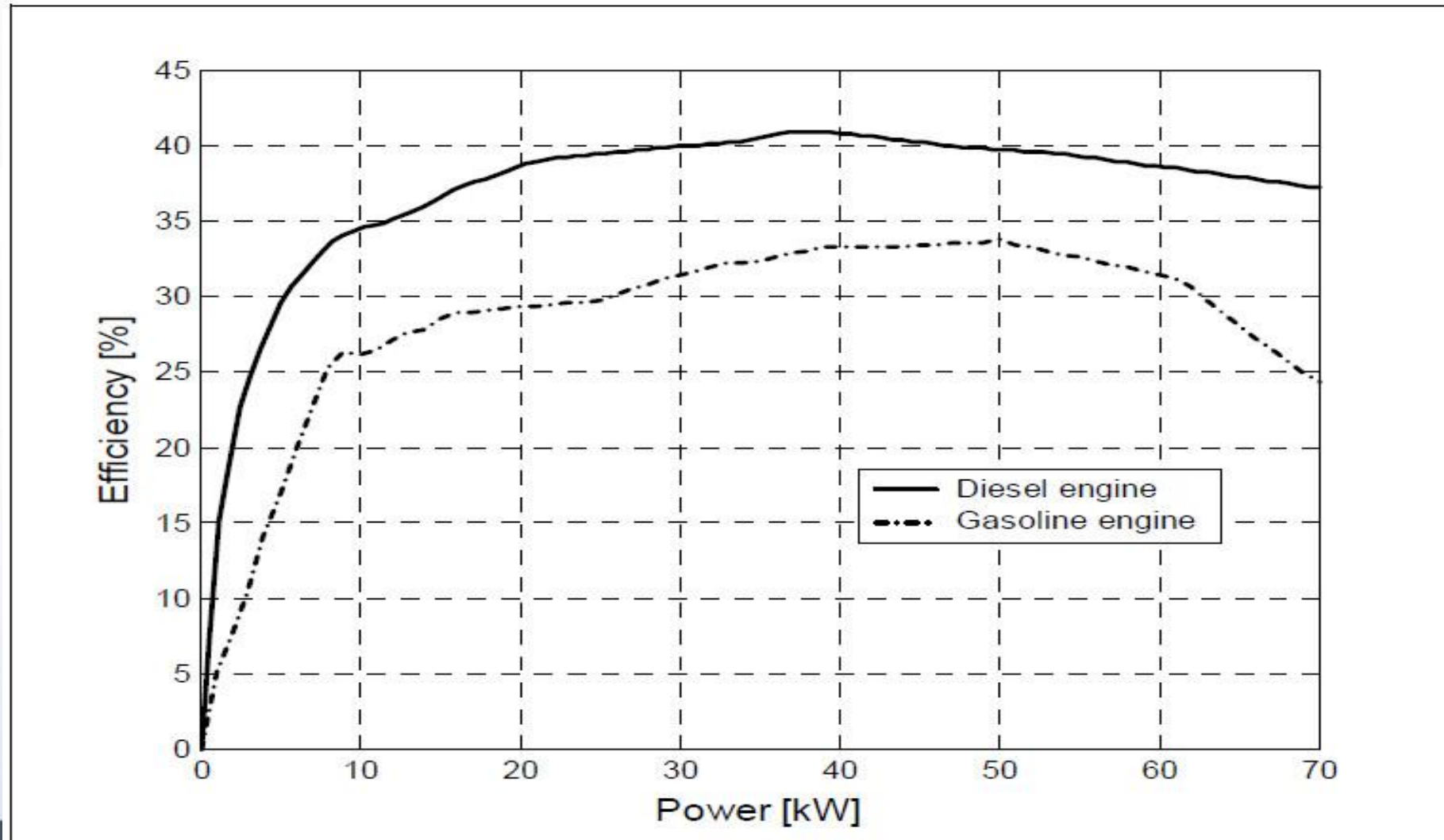
Graph power diesel and petrol engines
