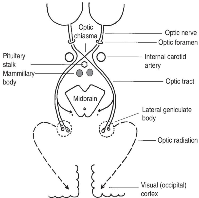
Fig. 20.1 Visual pathways.
